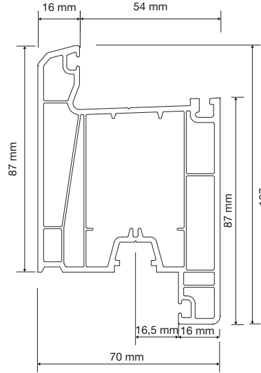
PR7S04B Kapı Profili Door Sash Profile
