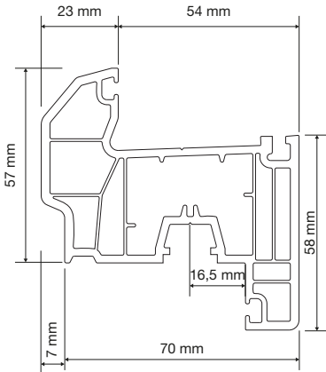
PR7S07 Damlalıklı Kanat Profili Drained Sash Profile
