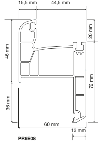
PR6E08 Pervazlı Kasa Profili Casing Frame Profile
