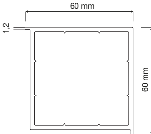
PR6034 60X60 Kutu 60X60 Box
