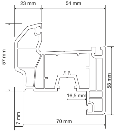
PR7S07 Damlalıklı Kanat Profili Drained Sash Profile
