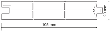
PRTS22 20x105 mm Lambri 20x105 mm Panel
