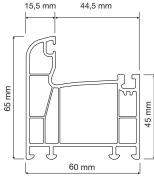
PR6E01 Kasa Profili Frame Profile
