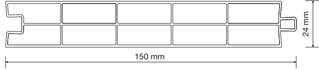
PRTS23 24x150 mm Lambri 24x150 mm Panel
