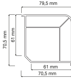
PR6S64 60x70 Kutu Profili 60x70 Box Profile
