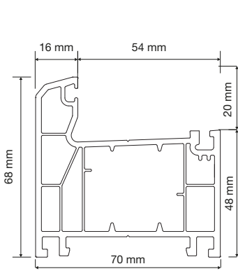
PR7V01B Kasa Profili Frame Profile
