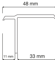
PRTS31 Asimetrik T T Covering
