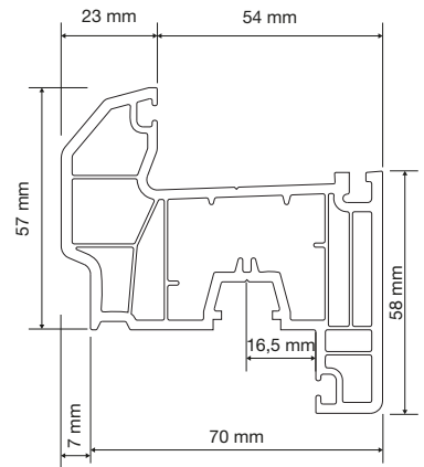
PR7S07 Damlalıklı Kanat Profili Drained Sash Profile
