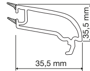
PR6E14B Oval Tek Cam Çıtası Oval Single Glazing Bead
