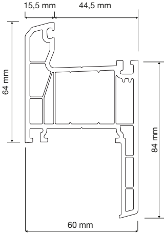
PR6S08 Pervazlı Kasa Profili Casing Frame Profile
