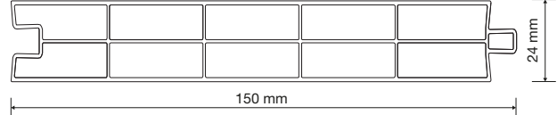
PRTS23 24x150 mm Lambri 24x150 mm Panel
