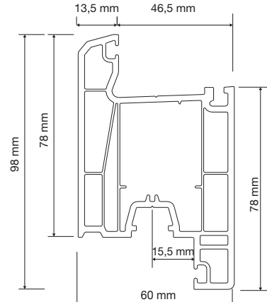
PR6E04B Kilitli Kapı Door Sash Profile
