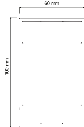
PR6034 60X100 Kutu 60X100 Box
