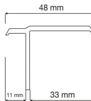
PRTS31 Asimetrik T T Covering
