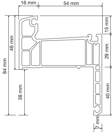
PR7S08 Pervazlı Kasa Profili Casing Frame Profile
