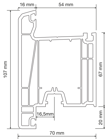
PR7V05B Kapı Profili Outside Opening Door Sash Profile
