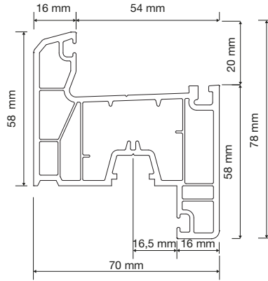
PR7V02B Kanat Profili Sash Profile
