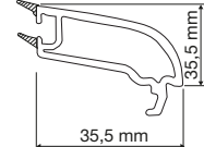
PR6E14B Oval Tek Cam Çitası Oval Single Glazing Bead
