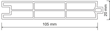
PRTS22 20x105 mm Lambri 20x105 mm Panel
