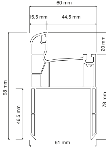
PR6E01 U Kasa Profili U Frame Profile
