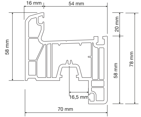
PR7S02 Kanat Profili (6 Odacıklı) Sash Profile (6 Chamber)
