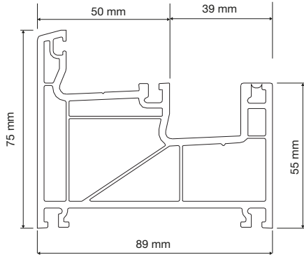
PRSL01 Sürme Tek Raylı Kasa Sliding Single Rail Frame
