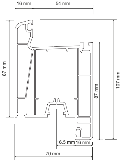
PR7V04B Kapı Profili Door Sash Profile
