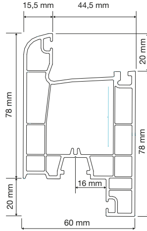
PR6E04 Kapı Profili Door Sash Profile
